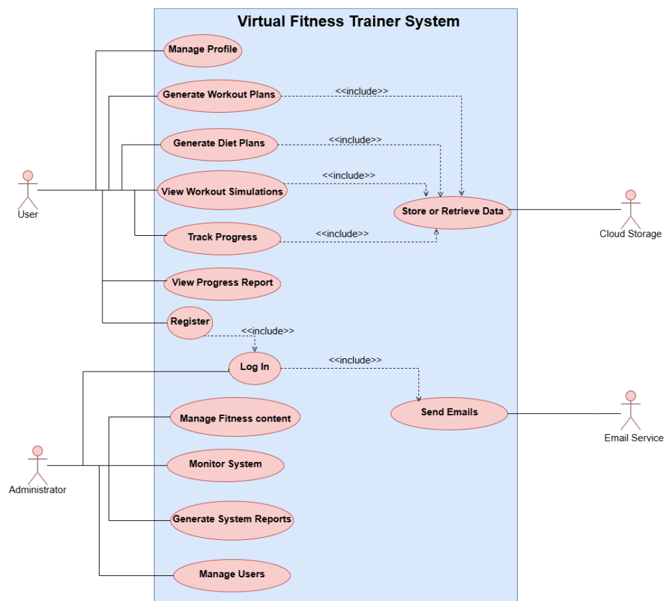
Figure 2: Use Case Diagram for Virtual Fitness Trainer
