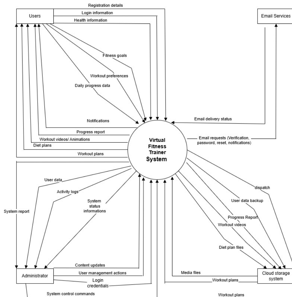
Figure 1: Context Diagram for Virtual Fitness Trainer
